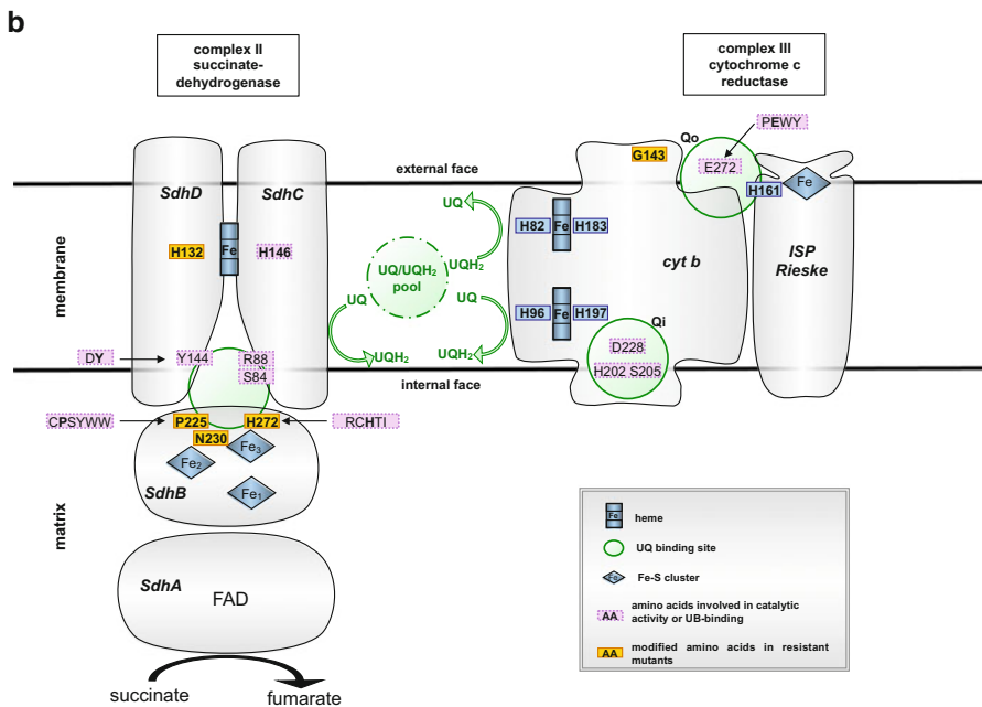
Fig. 10.1 Targets of respiration inhibitors and modified residues involved in resistance with focus on complex II inhibitors (SDHIs). (a) Enzyme complexes and target sites of respiration inhibitors on the electron transfer chain (Adapted from Leroux and Walker 2010); (b) Detailed view of complexes II and III of the ETC, with the conserved residues in the catalytic or ubiquinone ( UQ ) binding site (Adapted from Leroux and Walker 2010); (c) Chemical structure of some SDHIs (Adapted from Glättli et al. 2011); (d) Resistance profile of B. cinerea mutants to different SDHIs – field isolates (field) compared to sdhB site-directed mutants (lab). When particularly high SDHI concentrations are necessary to determine the EC_{50} value, only the minimum resistance factors are indicated over the columns (>RF) (Adapted from Lalève et al. 2014b)
